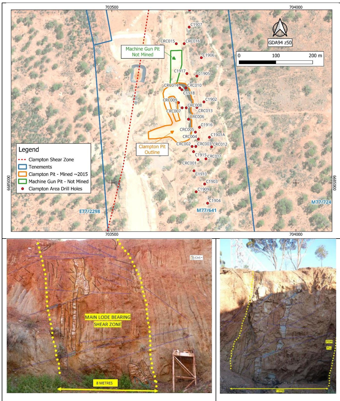
Figure 5.3: Clampton prospect – plan of historical workings and drilling (upper) with photographs of the main lode-bearing shear zone (lower)
