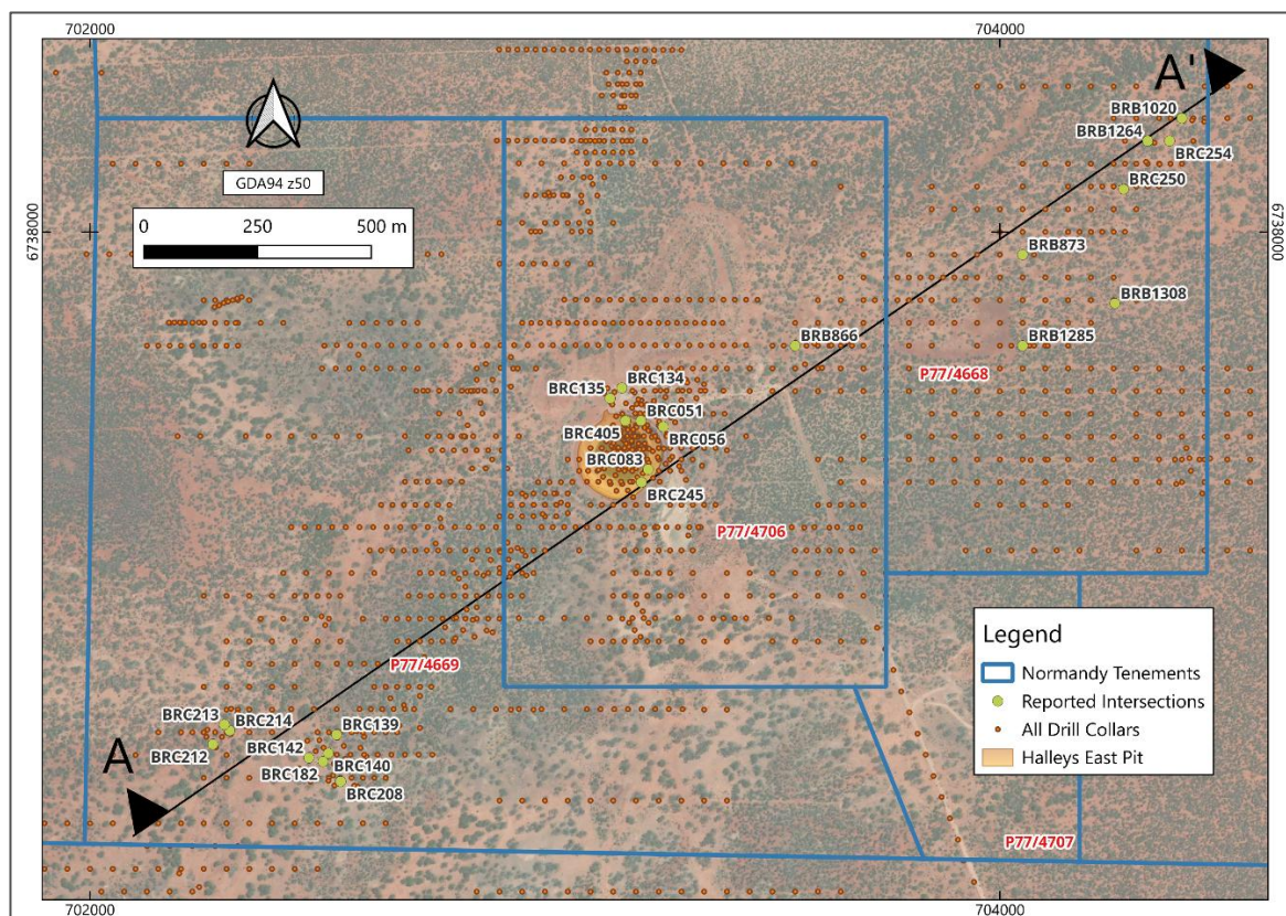
Figure 4.9: Drill hole collars around Halley's East Pit
