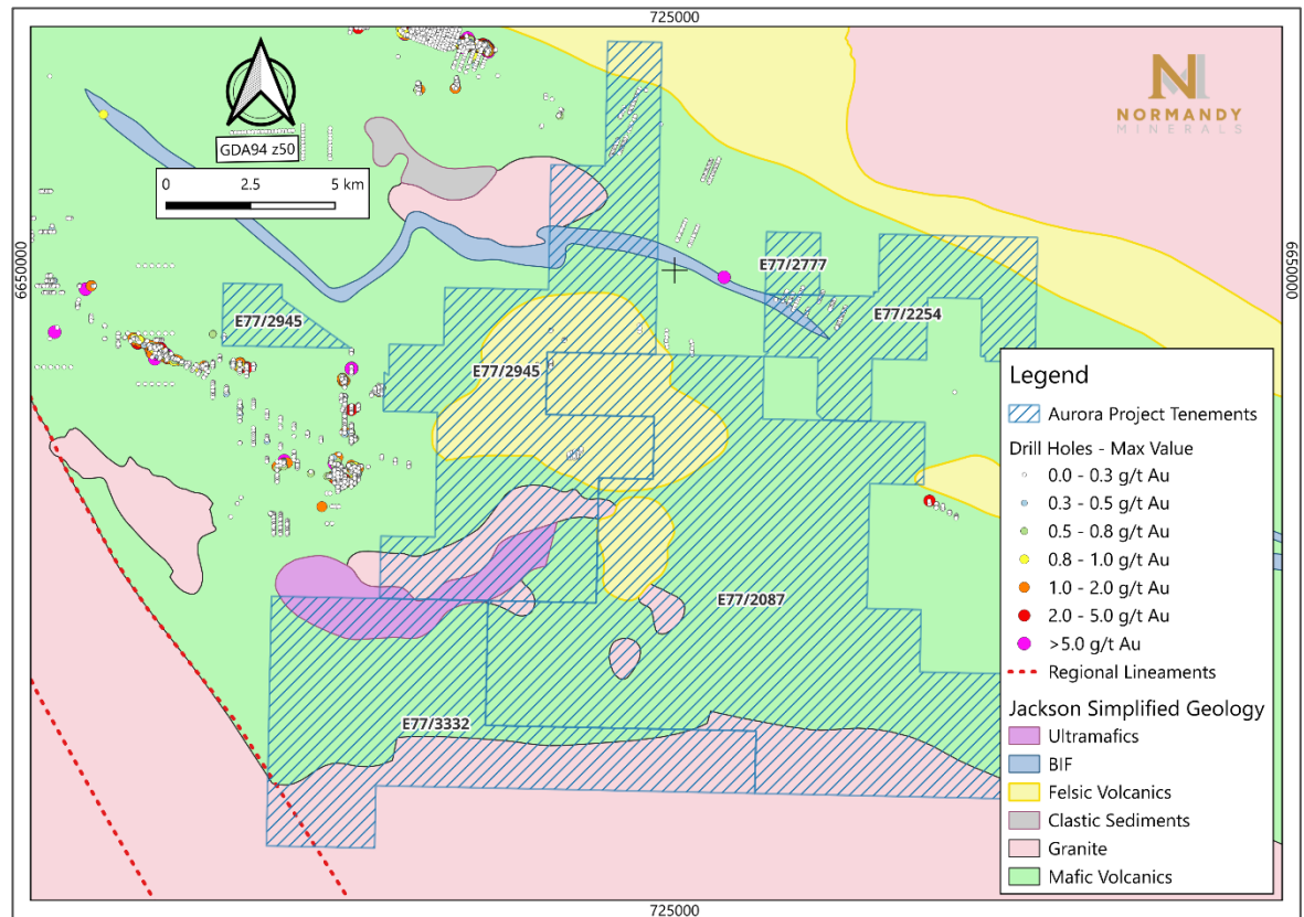
Figure 5.24: Historical drilling surrounding the Aurora prospect
