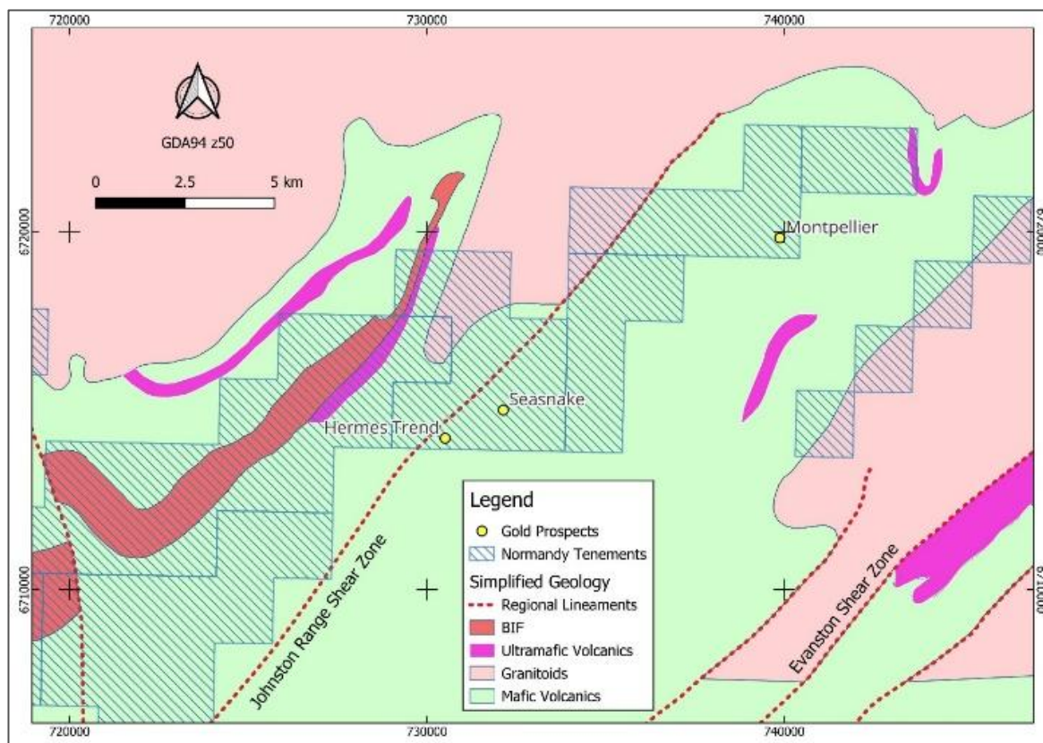
Figure 4.16: Location of Hermes Trend
