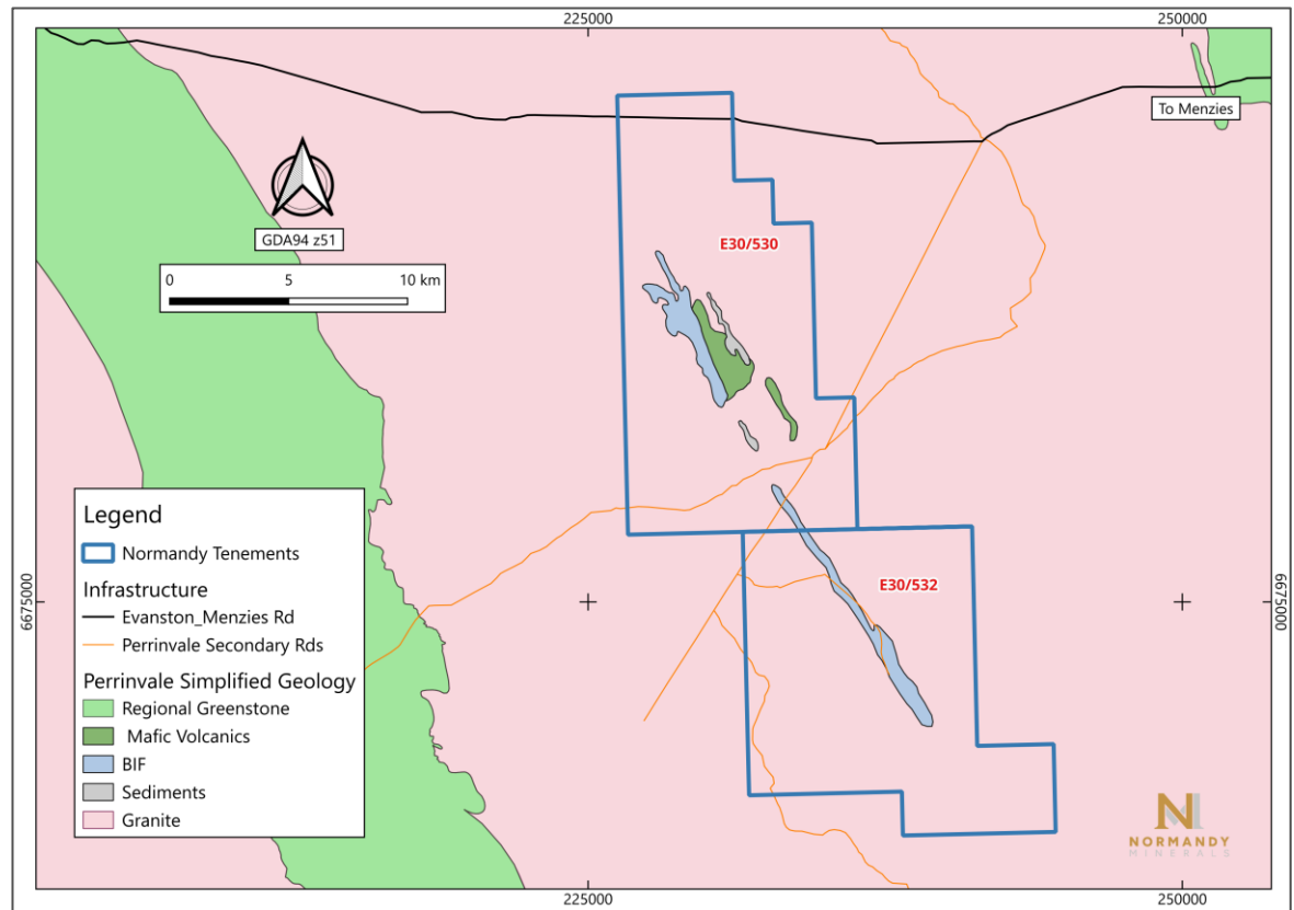
Figure 6.1: Simplified bedrock geology map of the Perrinvale Project area
