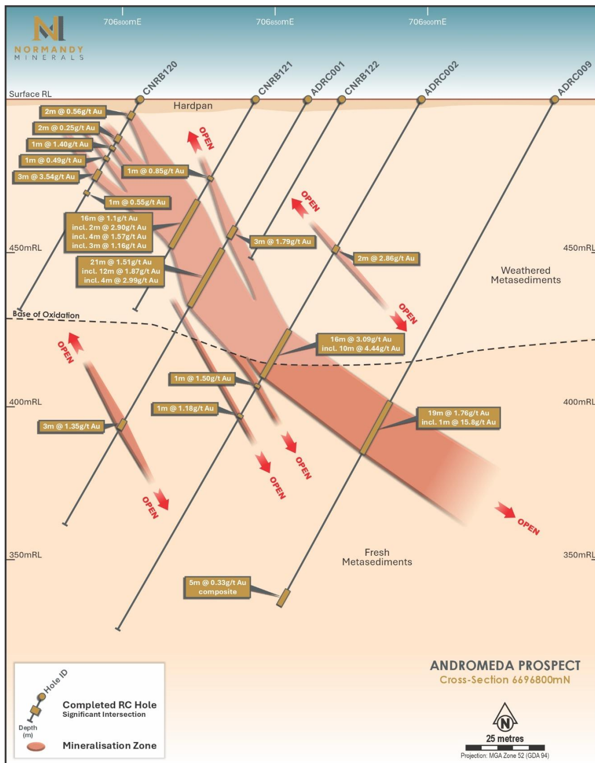
Figure 5.11: Conceptual section of Andromeda Prospect
