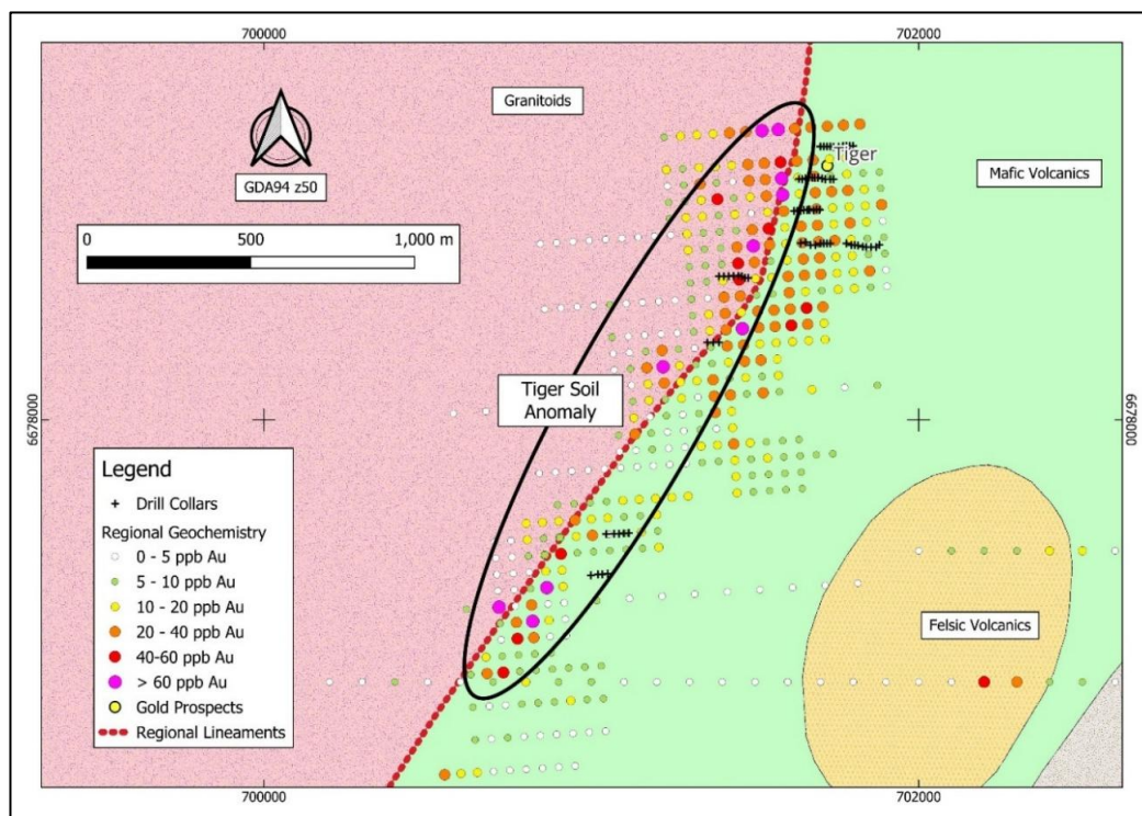
Figure 5.16: Soil anomaly and drill holes in the Tiger prospect
