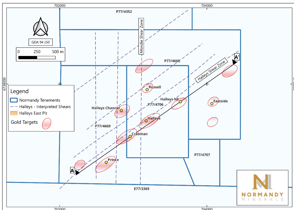
Figure 4.8: Schematic representation of shallow drilling interpreted structures around Halley's East Pit
