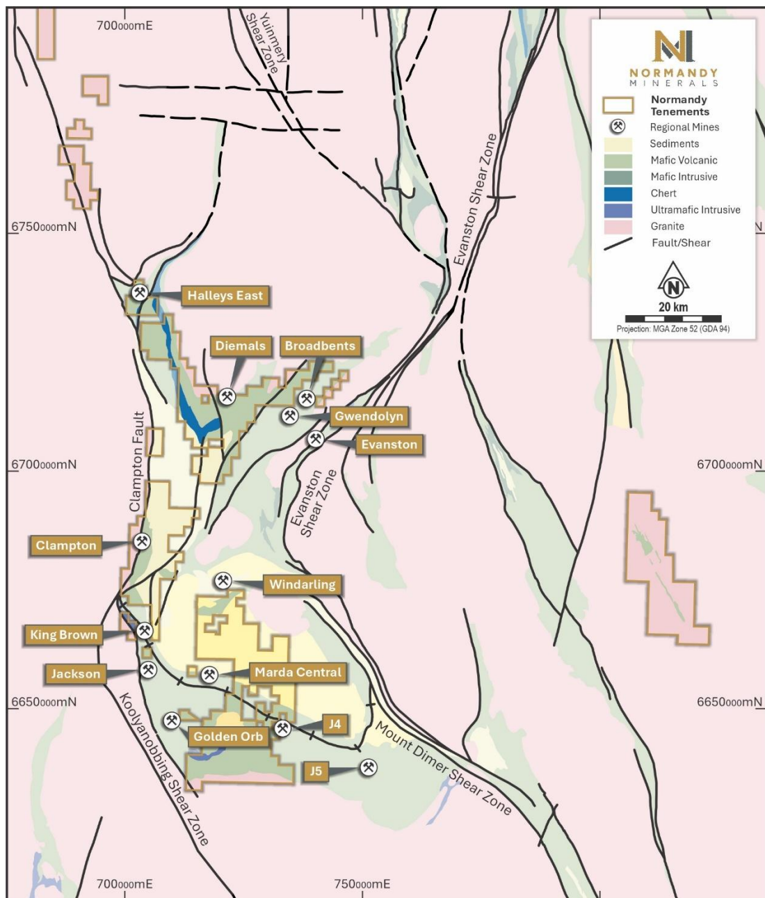
Map 3: Normandy tenure and existing mines within region
