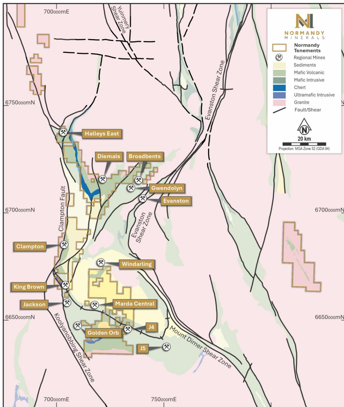
Figure 3.1: Regional geological map of Normandy's tenure
