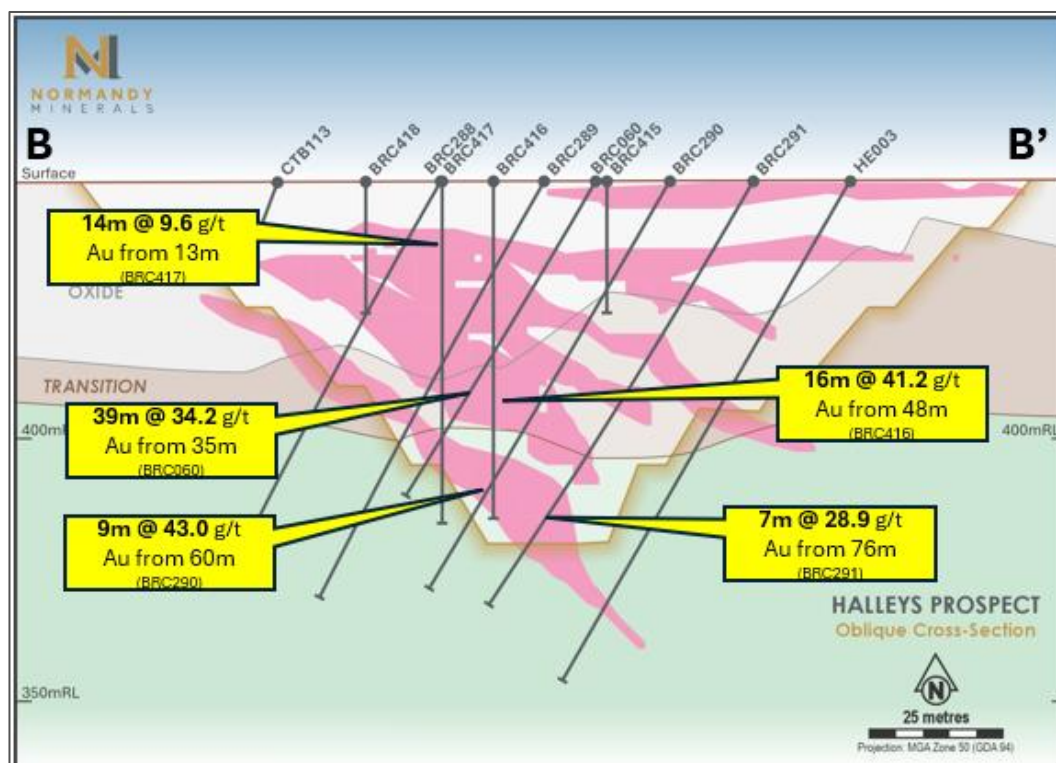
Figure 4.5: Cross section B–B' of Halleys East Pit*
