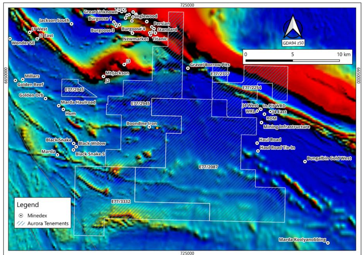
Figure 5.21: Aurora tenement area over regional total magnetic intensity imagery and historical mines and prospects
