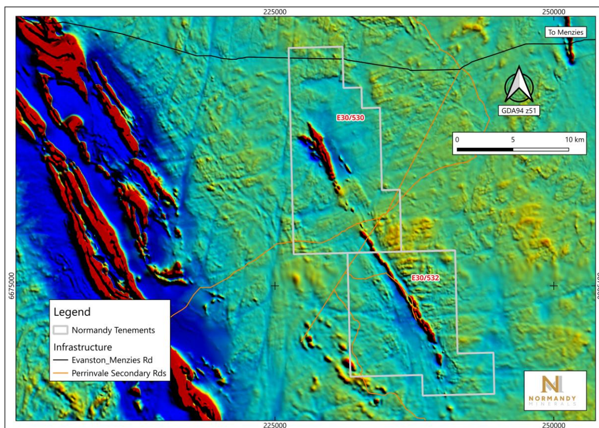
Figure 6.2: Airborne total magnetic intensity map of Perrinvale Project area
