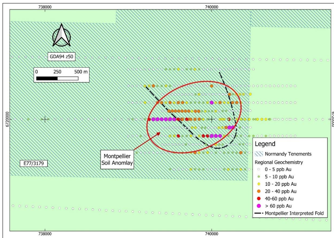
Figure 4.17: Soil anomalies in Montpellier
