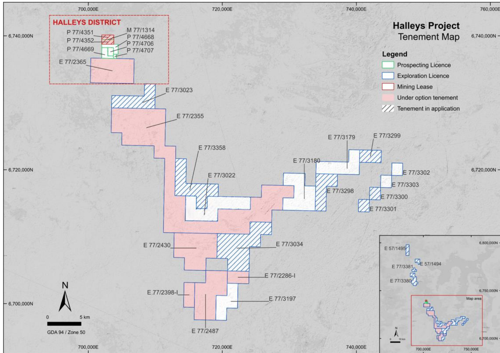
Figure 4.1: Tenement layout of Halleys Project
