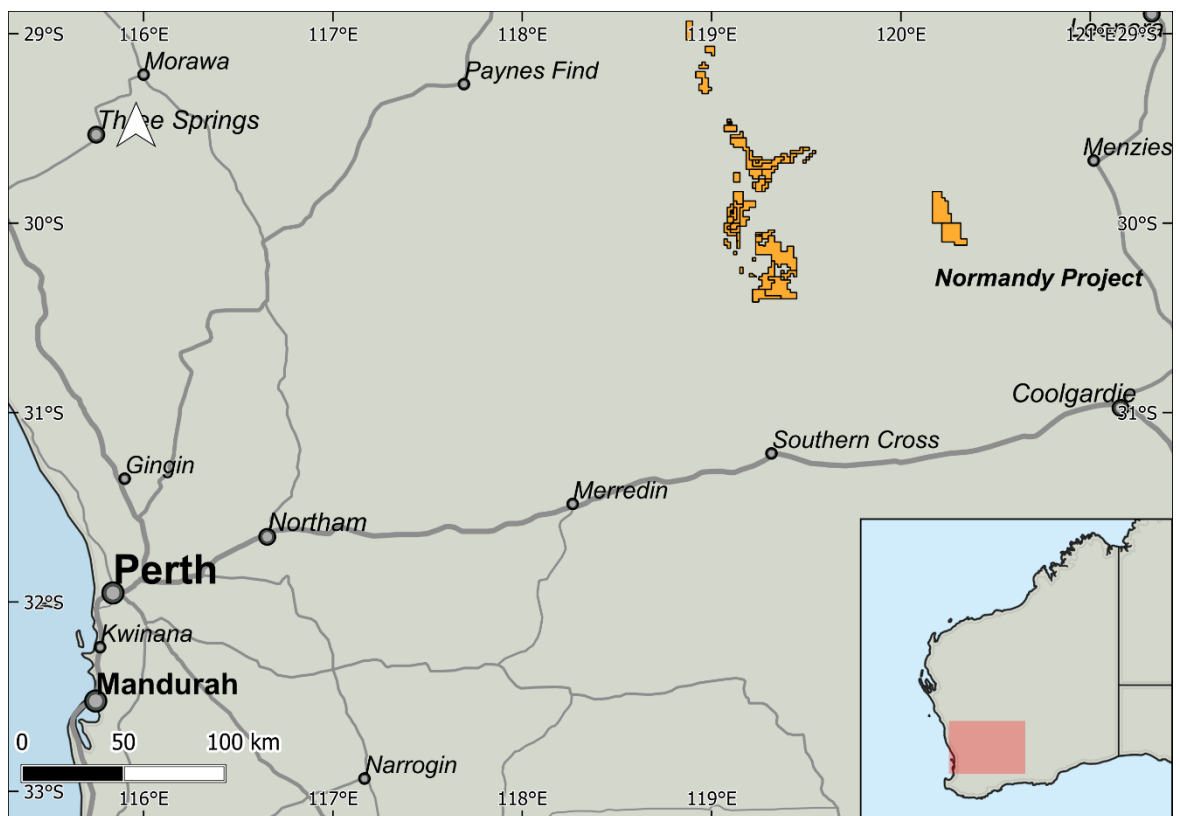
Figure 2.1: Location of the Normandy Project
