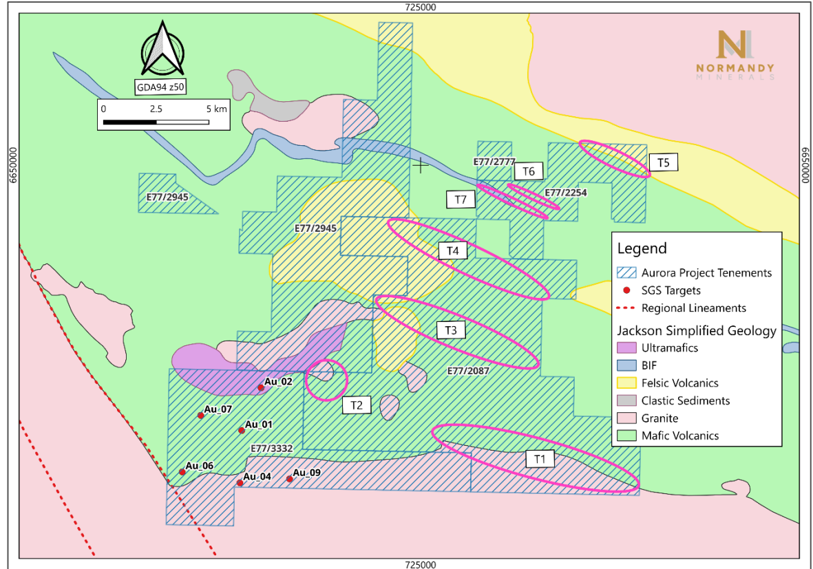
Figure 5.22: Aurora targets identified in historical exploration
