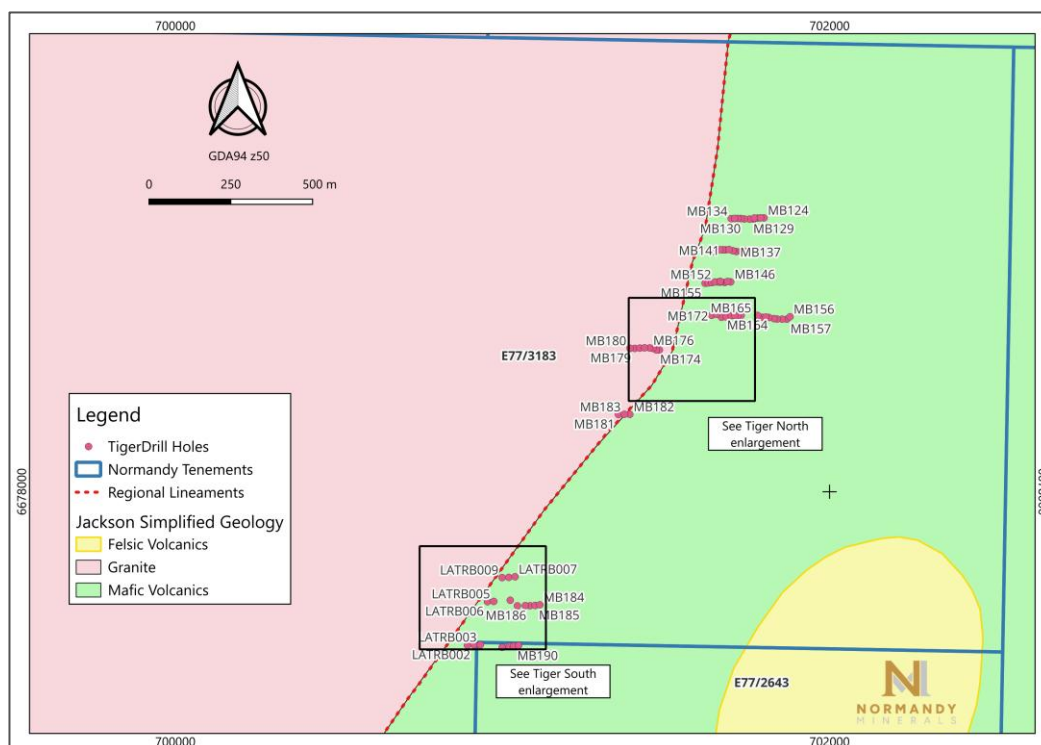
Figure 5.17: Historical drill holes in Tiger area
