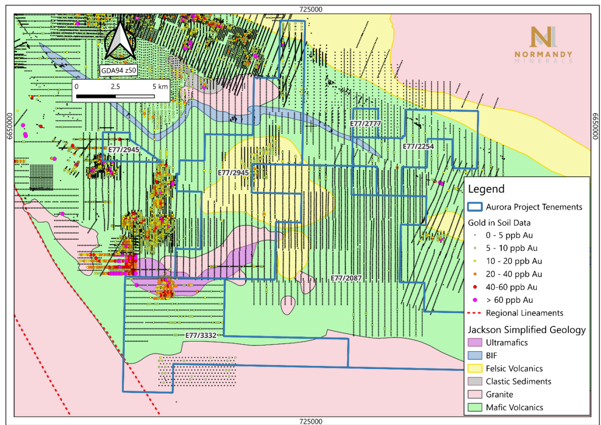
Figure 5.23: Soil sampling results surrounding the Aurora prospect
