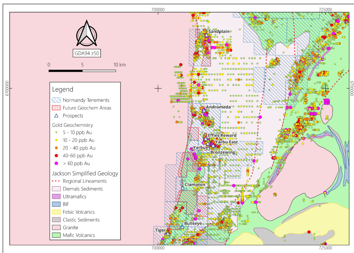
Figure 5.2: Regional gold-in-soil anomalies in Clampton Shear Zone and proposed soil geochemical survey areas
