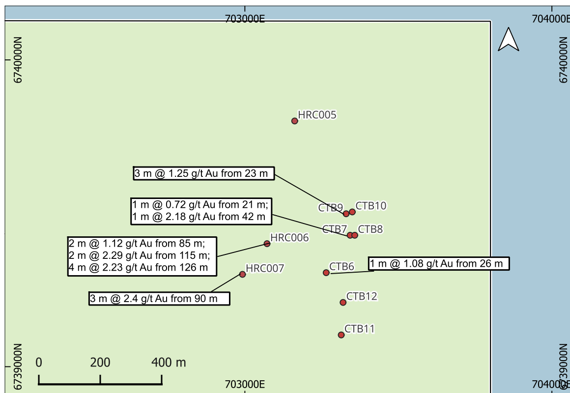
Figure 4.11: Drill holes with significant intercepts within the Phil prospect
