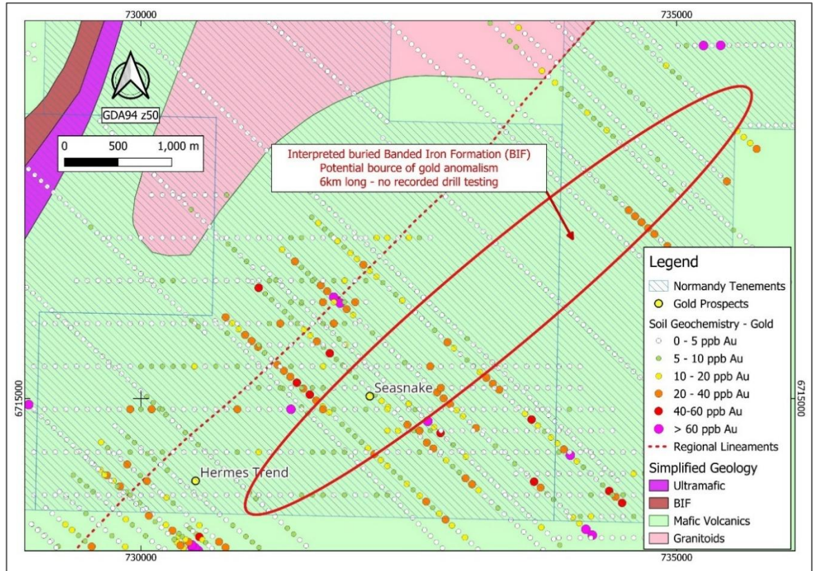
Figure 4.19: Soil anomalies in Seasnake
