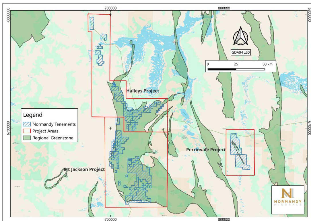
Figure 2.2: Normandy Tenements layout
