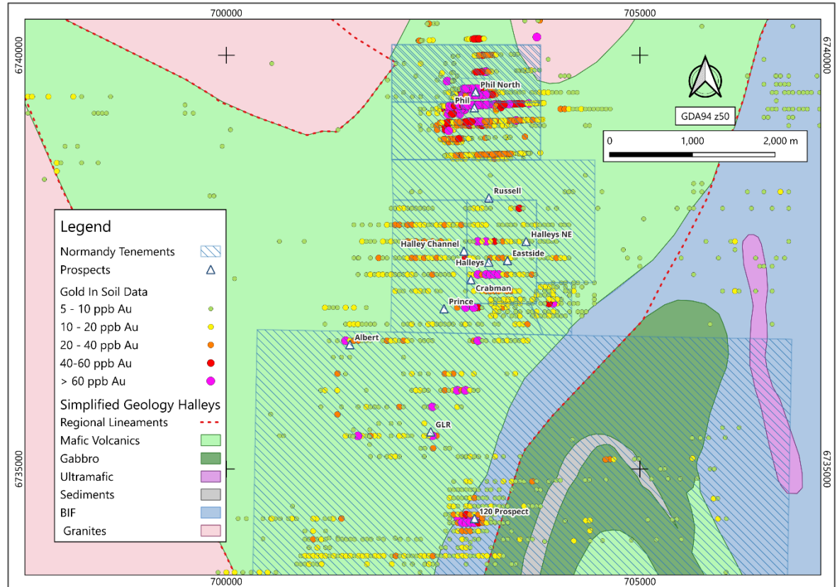
Figure 4.2: Regional gold-in-soil anomaly in Halley's District
