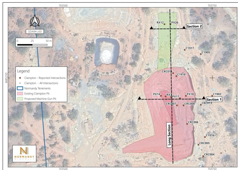
Figure 5.6: Historical drill holes location in Clampton prospect
