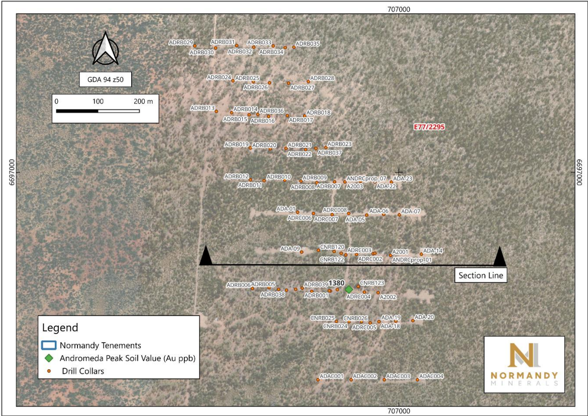
Figure 5.10: Drill hole collars in Andromeda prospect
