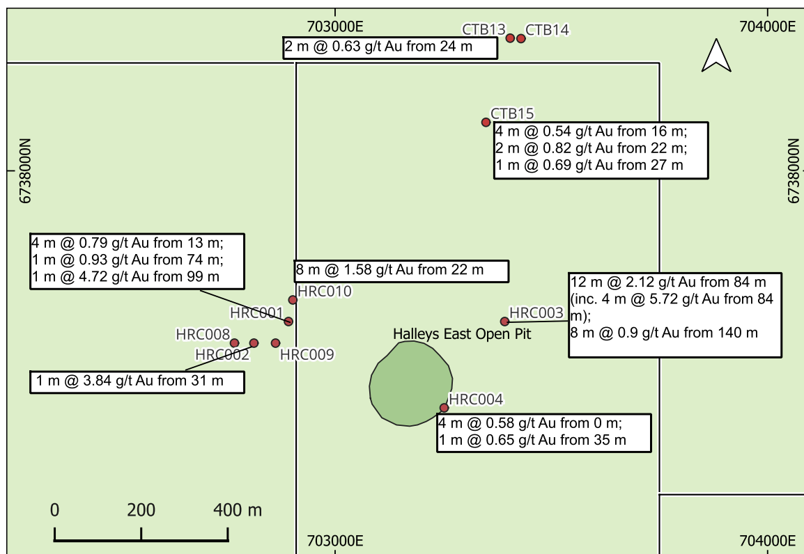
Figure 4.6: Drill holes with significant intercepts surrounding Halley's East Pit
