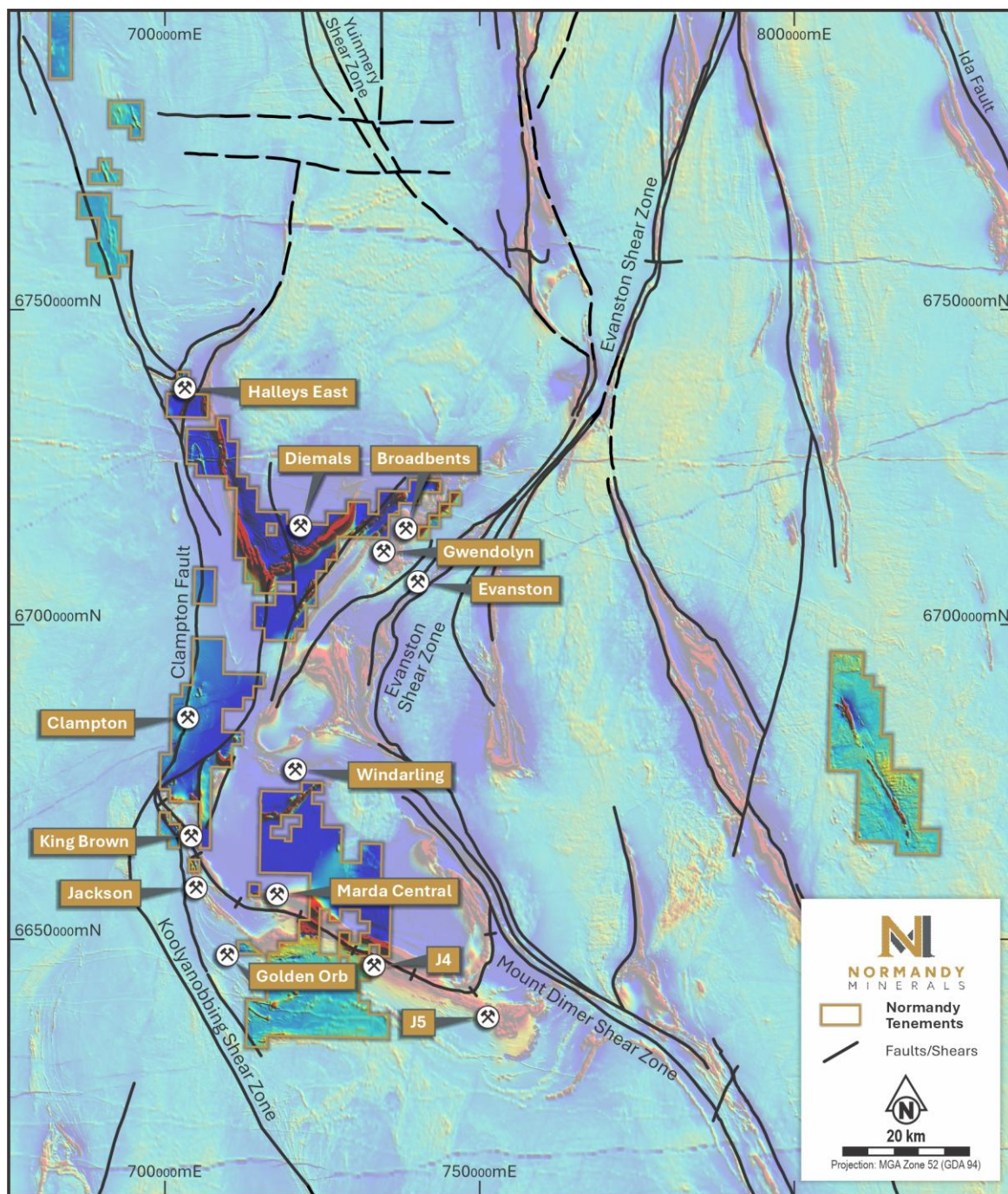
Figure 3.2: Regional airborne total magnetic intensity map of Normandy's tenure
