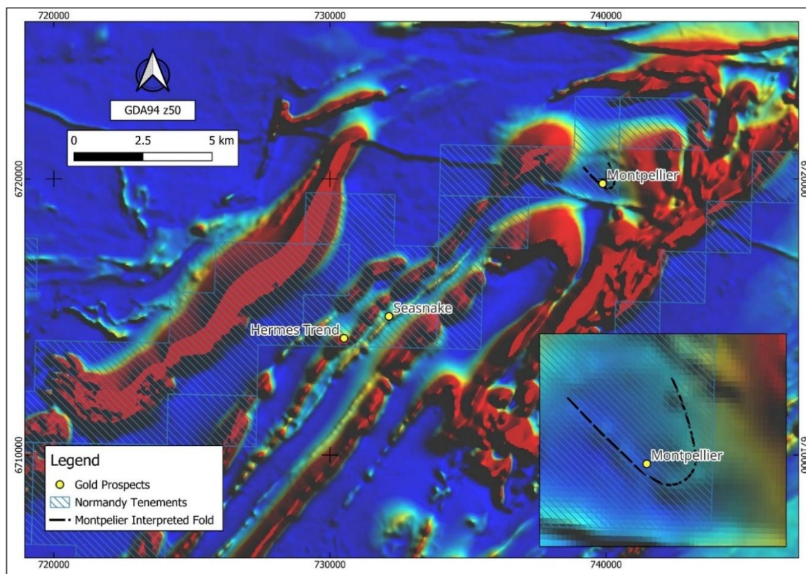
Figure 4.18: Total magnetic intensity imagery of the Hermes Trend area
