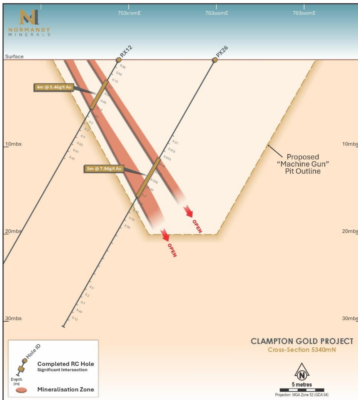
Figure 5.8: Schematic cross section 2 along proposed Machine Gun Pit, looking north
