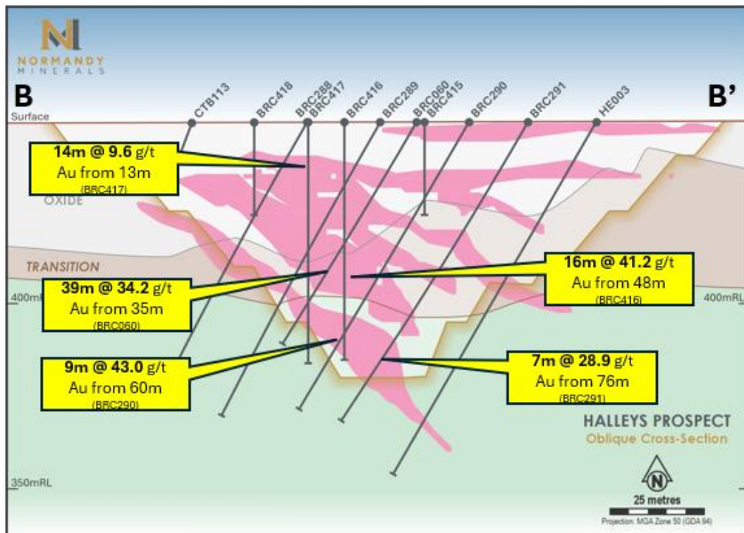
Figure 5.2: Cross section B-B' of Halley's East Pit
