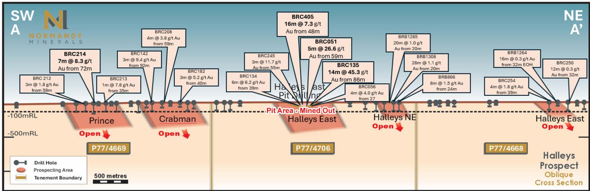
Figure 4.10: Schematic long section across various prospects through Halleys East Pit area
