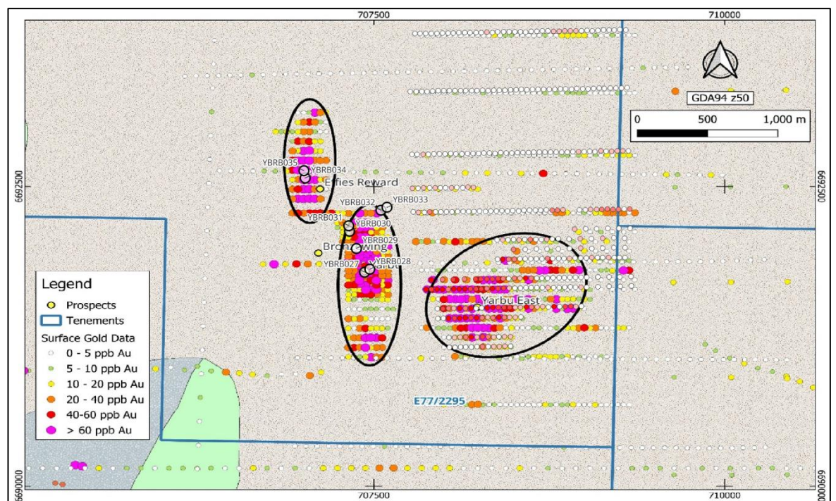
Figure 5.12: Soil anomalism and drill hole collars at Yarbu
