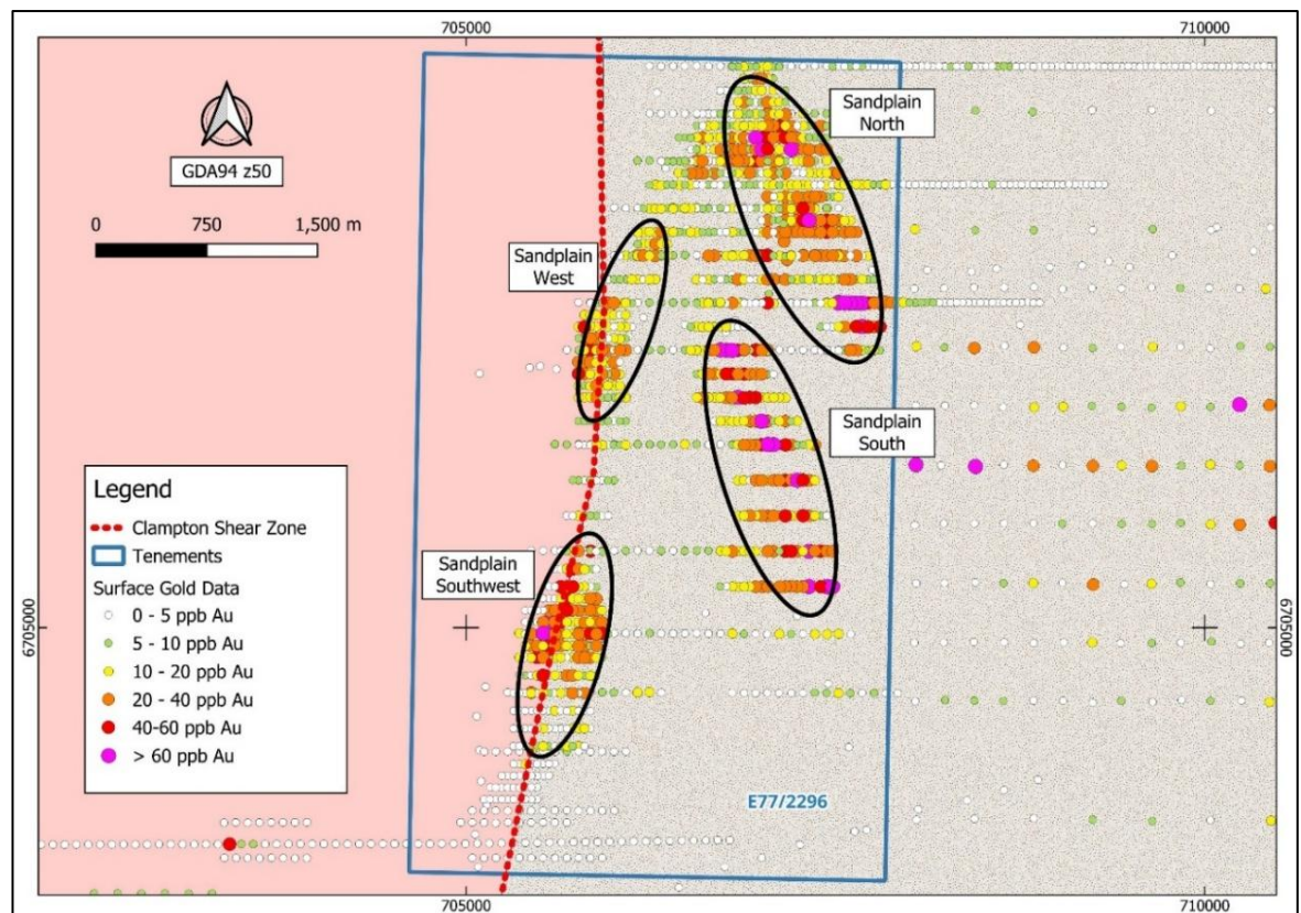
Figure 5.14: Soil anomalism in the Sandplain area
