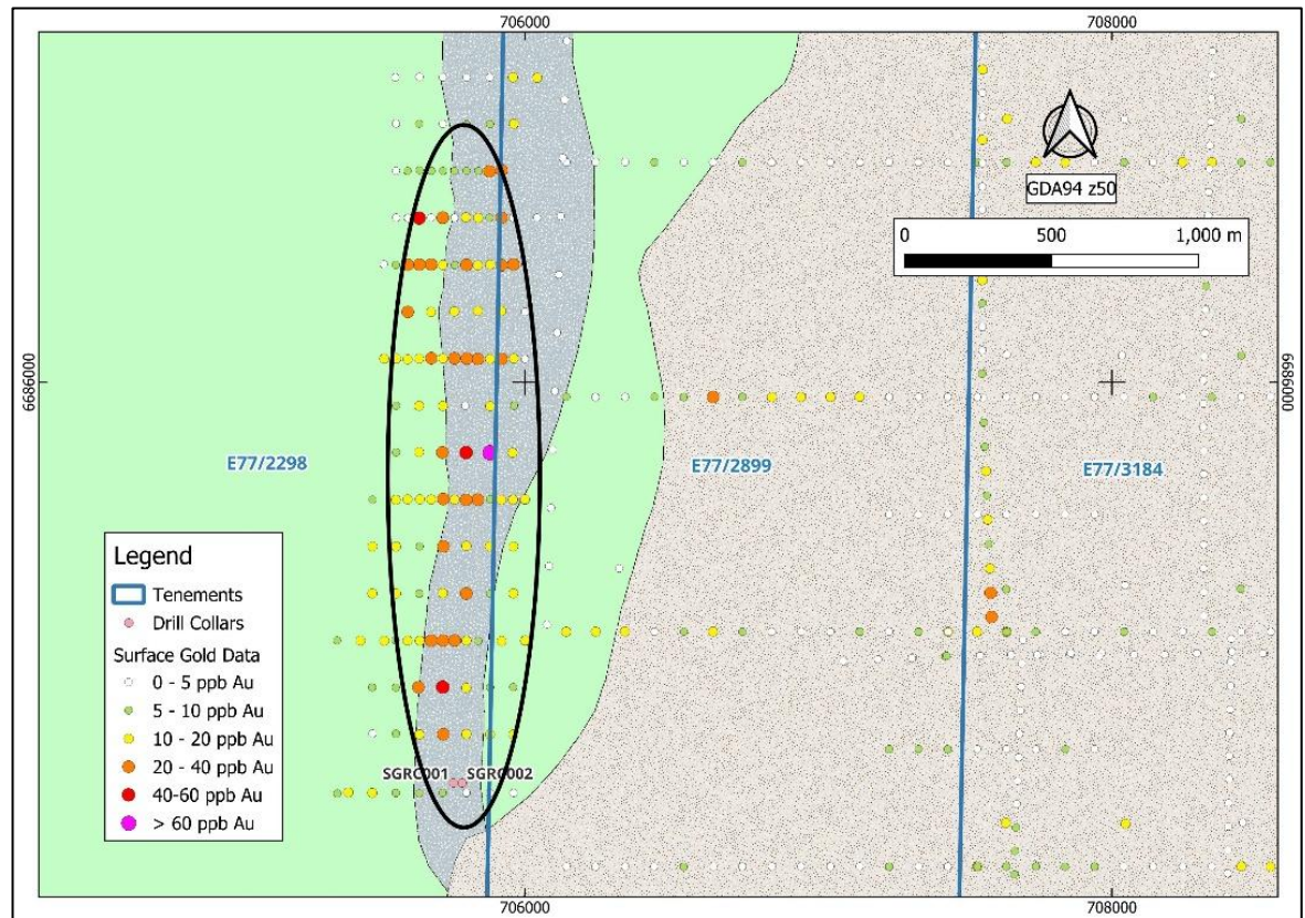
Figure 5.18: Soil anomaly in Gossan East
