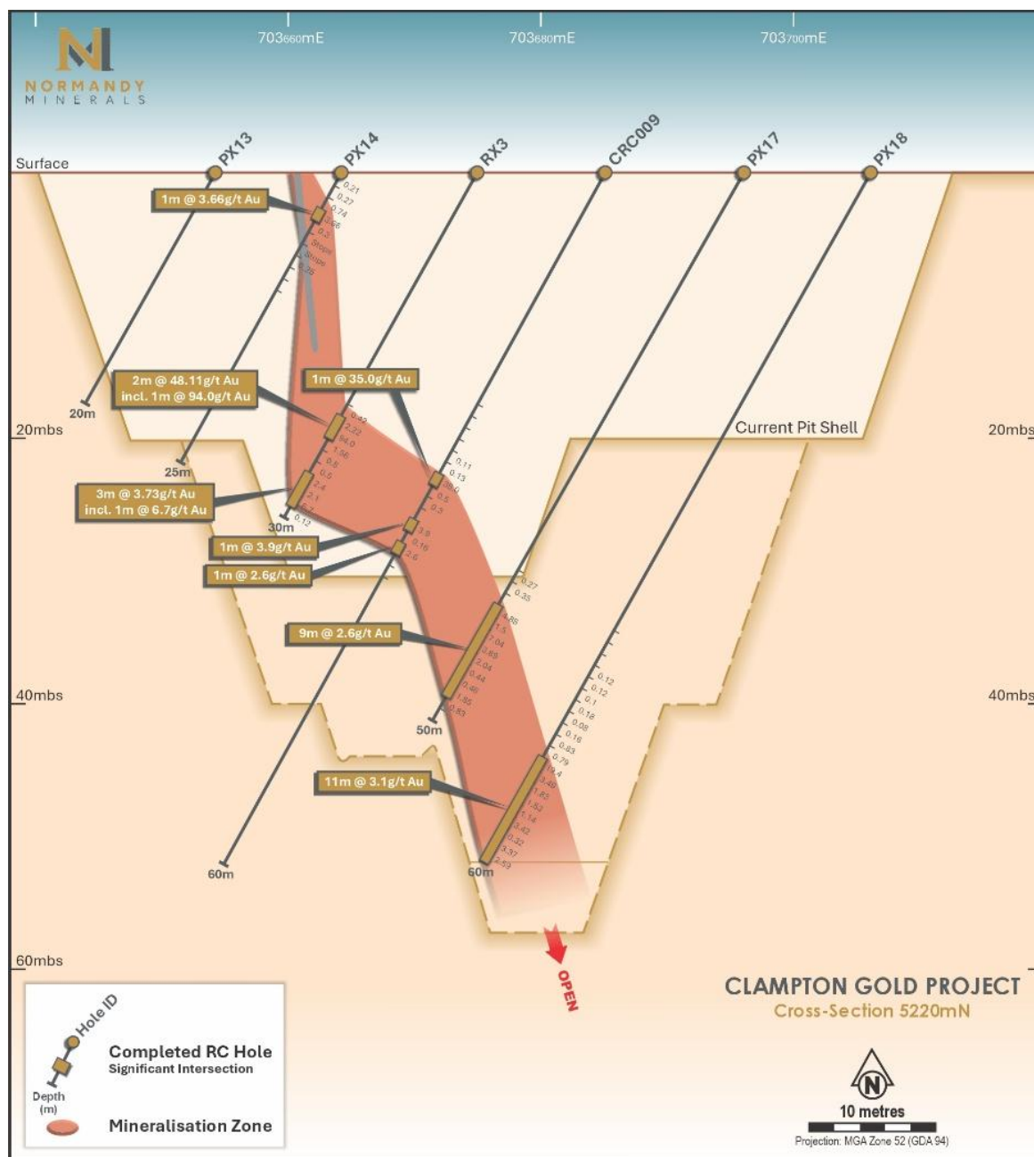
Figure 5.7: Schematic cross section 1 along Clampton Pit, looking north
