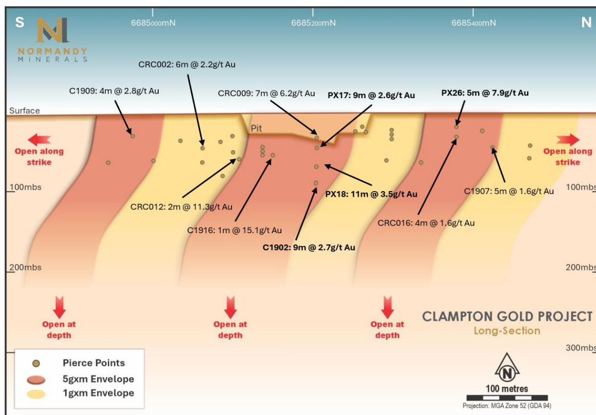
Figure 5.9: Schematic long section along strike of Clampton Pit showing significant drill hole pierce points, looking west
