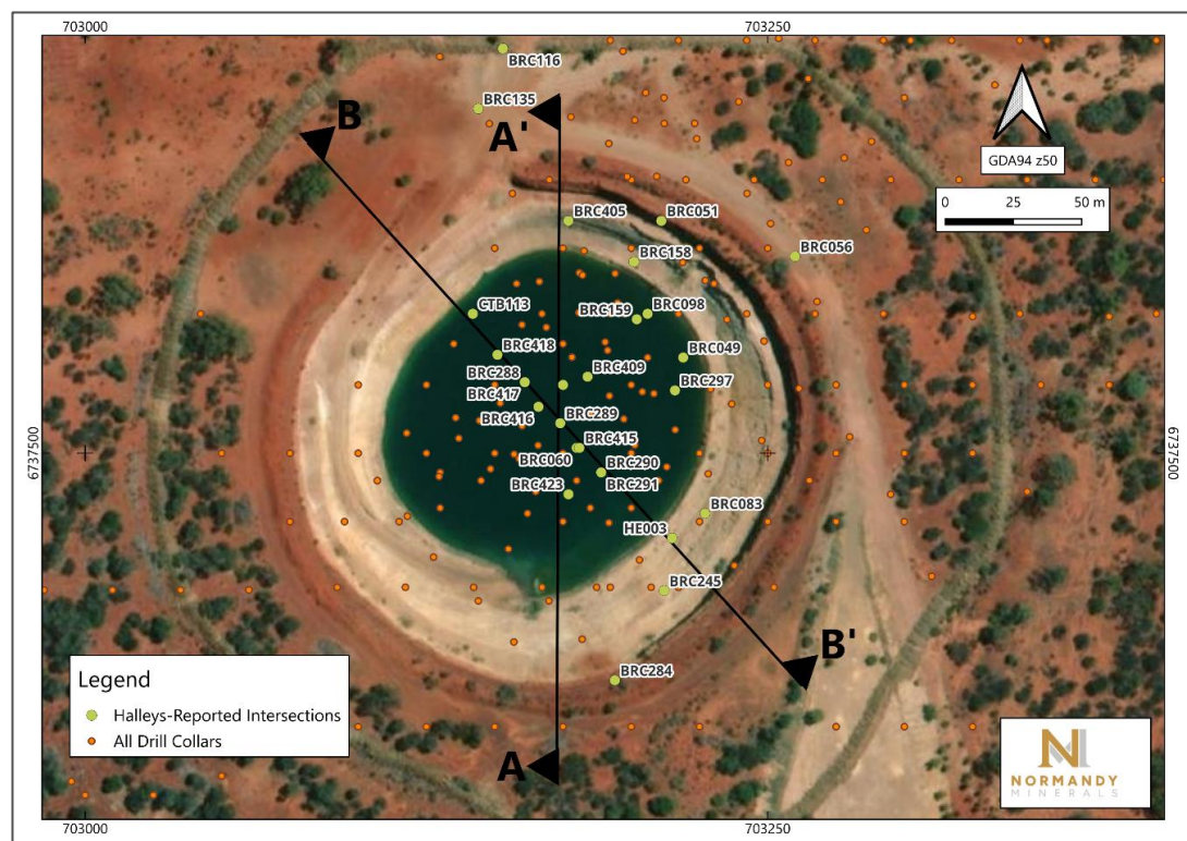
Figure 4.3: Drill hole layout surrounding Halleys East Pit*
