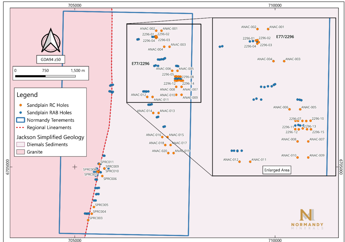
Figure 5.15: Historical drill hole collars at Sandplain
